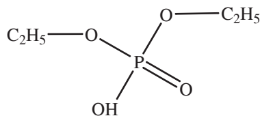
diethyl acid phosphate
