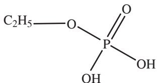
monoethyl acid phosphate
